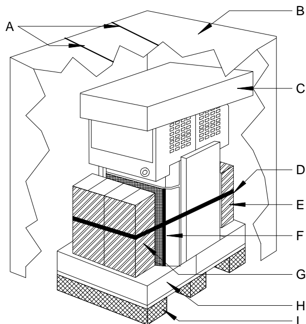
FIGURE 1 Unit Package
