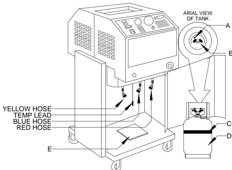
FIGURE 3 TANK INSTALLATION
