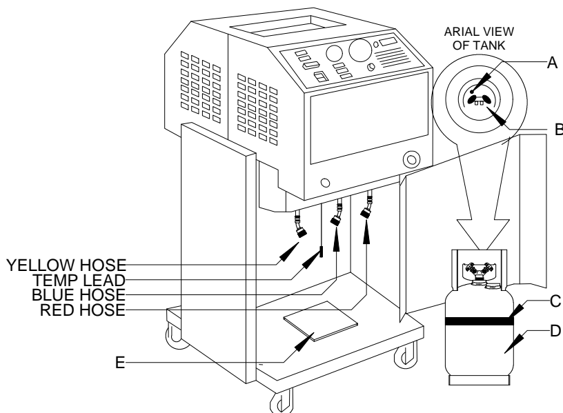
FIGURE 5 TANK INSTALLATION
