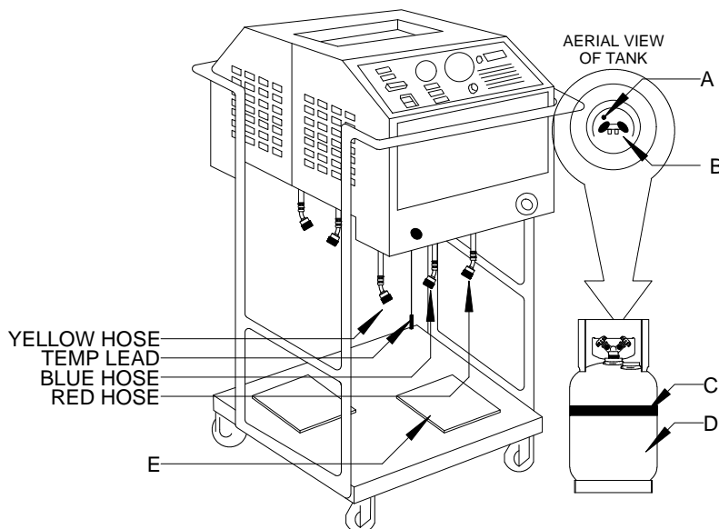
FIGURE 5 TANK INSTALLATION
