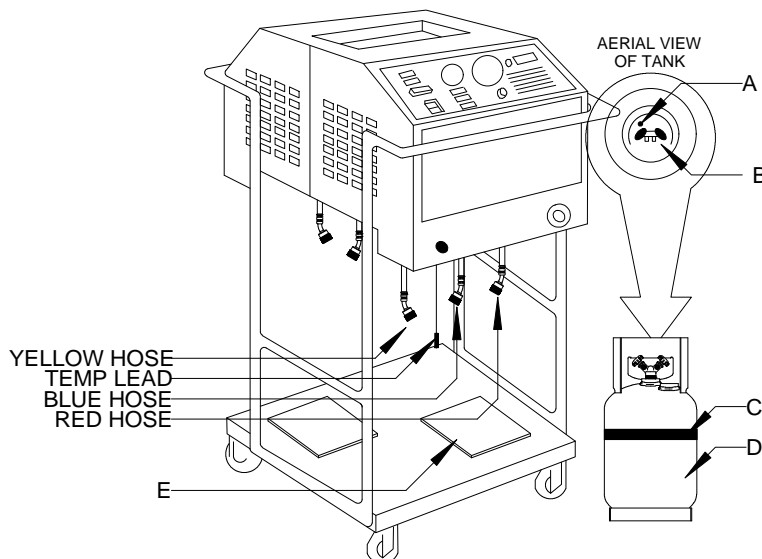
FIGURE 3 TANK INSTALLATION
