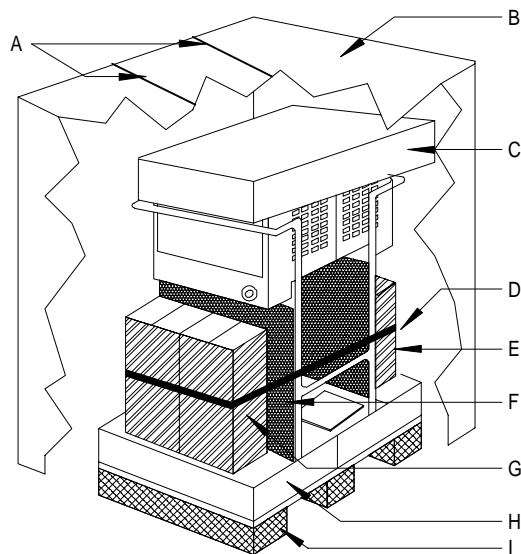
FIGURE 1 Unit Package
