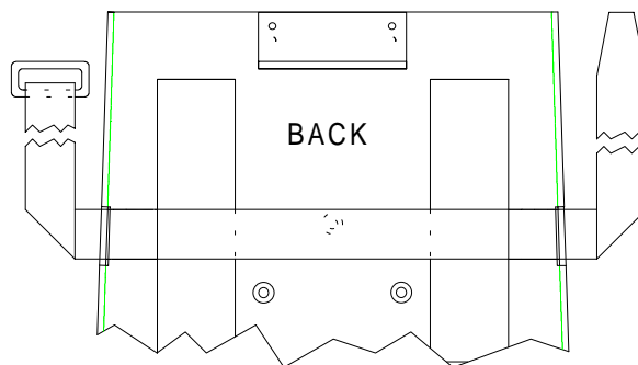
Figure 2, Monitor Base Plate for 15" Sampo Monitor.
