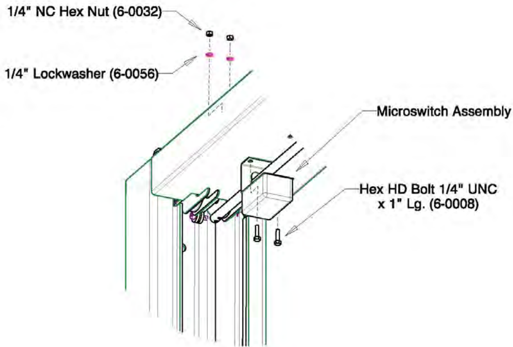
Figure 9: Mounting Microswitch
