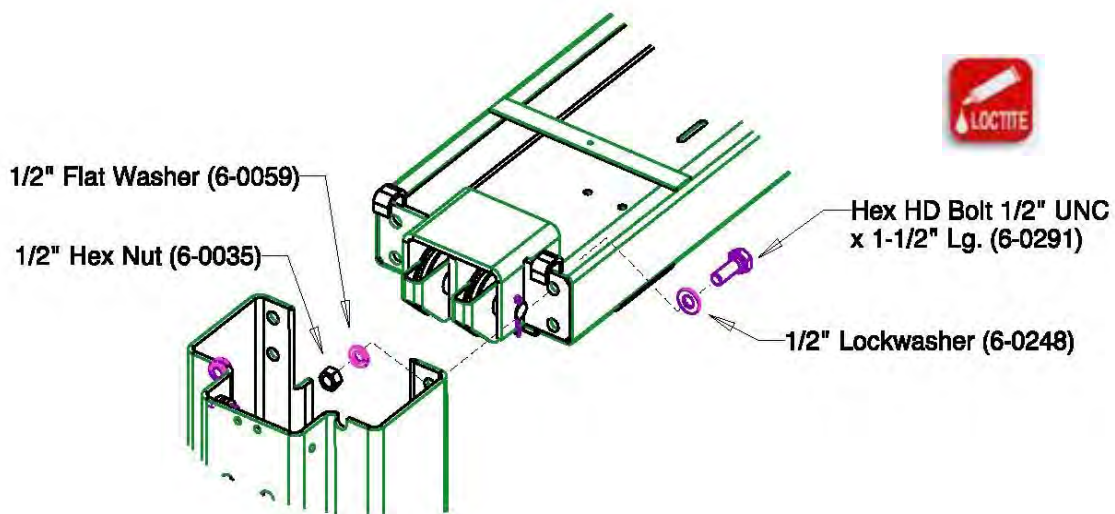
Figure 6 – Crossmember Assembly
