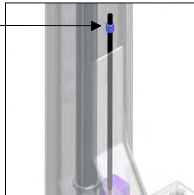
Transparent view of Carriage from Front.
