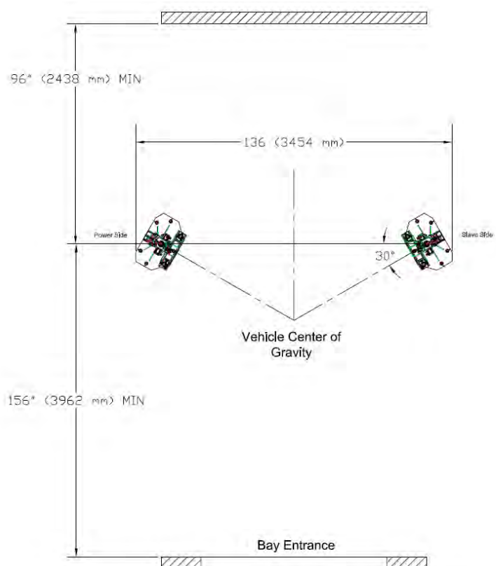
Figure 4. Bay Layout
