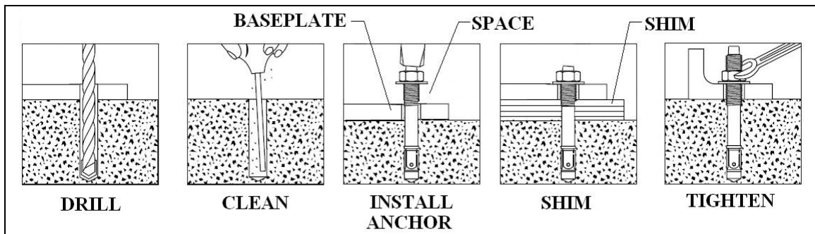
Figure 12. Anchor installation
