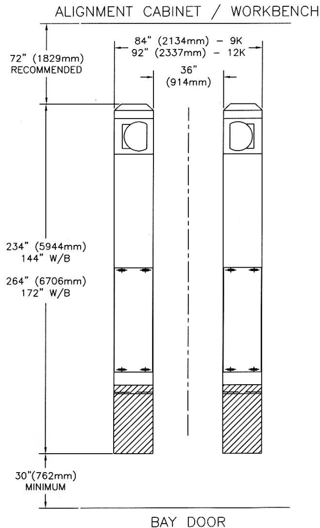
Figure 2 - Typical bay layout (surface mount)
