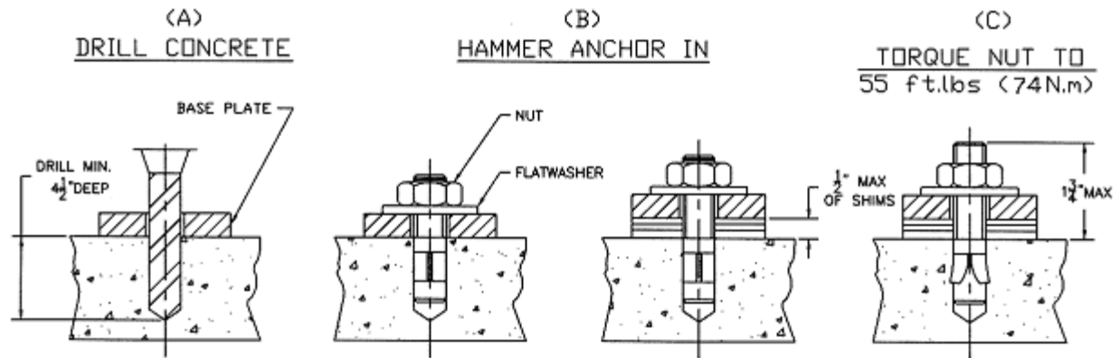
Figure 9 - Anchoring
