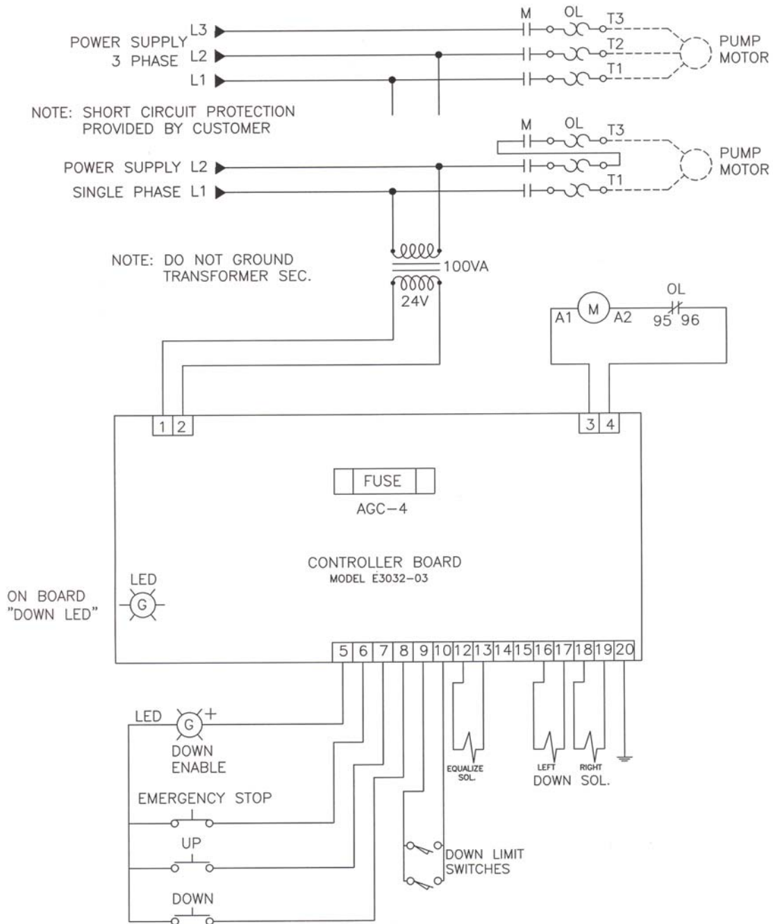
Figure 5 - Electrical Schematic; 220 Volt, 3Ph.
