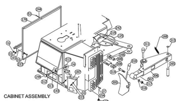
CABINET ASSEMBLY
