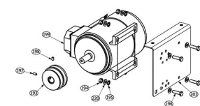
MOTOR & PULLEY 2 SPEED
