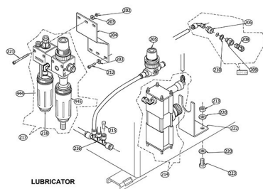
LUBRICATOR
