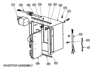
INVERTER ASSEMBLY
