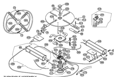
TURNTABLE ASSEMBLY
