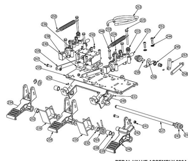
PEDAL VALVE ASSEMBLY 326A
