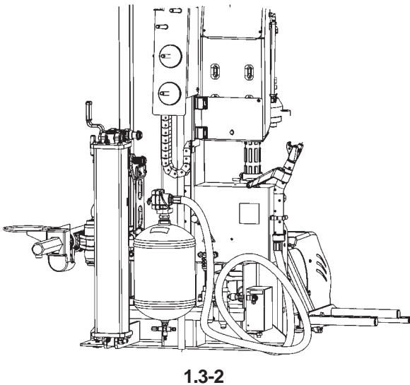
Figure 1-3.2 Represents the same machine as above, but it is also equipped with a beading unit for tubeless tires.
