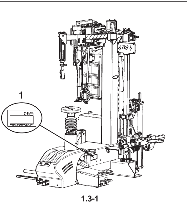
Figure 1-3.1 Represents the basic machine with automatic Head (integrated lever).
