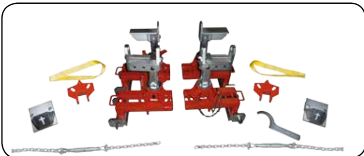
Optional Anchoring System for Chassis Type Vehicle and Four Wheel Drive (BHPLT19US)
